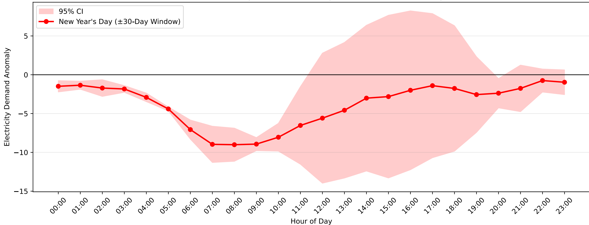
Sefton Demand Anomaly: New Year's Day (2010-2011, \pm 30 -Day Window)
